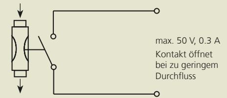
TBi beCool 2.2 Sensor
