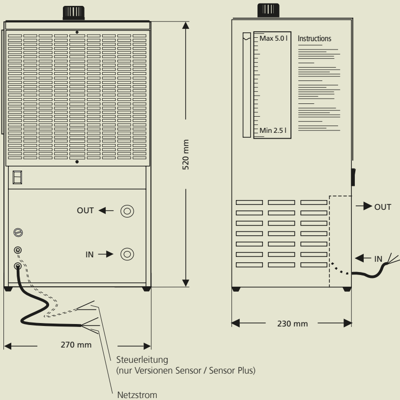
TBi beCool 2.2 Sensor
